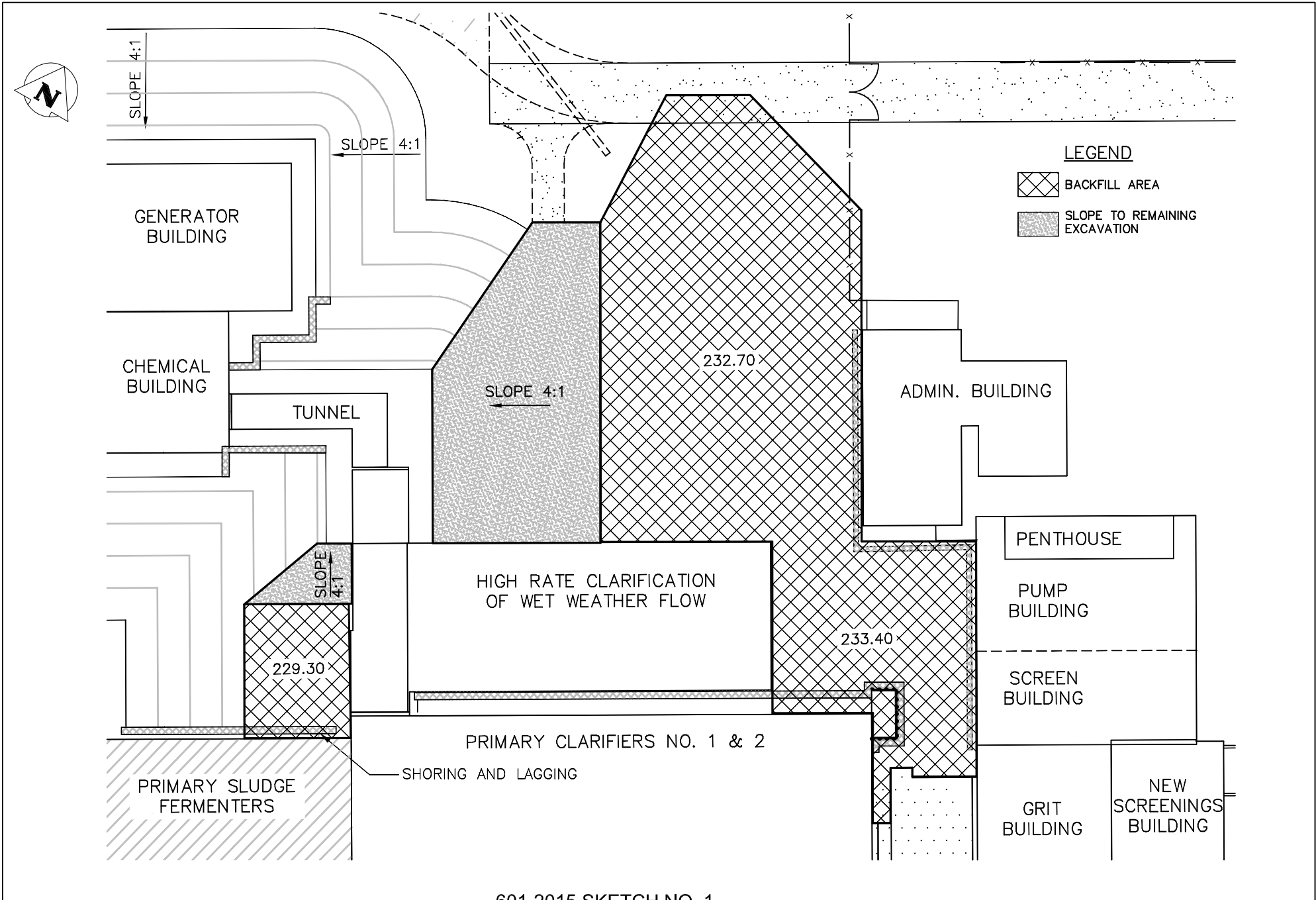
601-2015 SKETCH NO. 1 BACKFILL LIMITS
